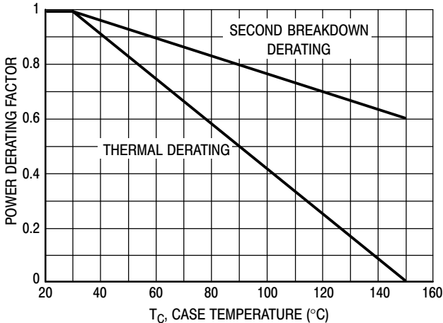
Figure 21. Forward Bias Power Derating
